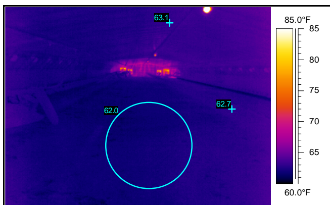
Figure 2. Thermal image of house using side wall inlets between flocks (springtime).
