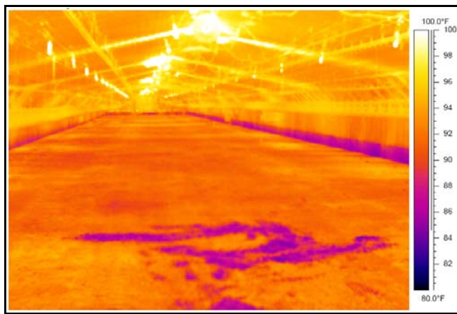
Figure 5. Thermal image of house using attic inlets between flocks (summertime).
