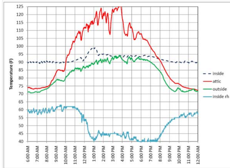
Figure 6. Temperatures in a broiler house using attic inlets during hot weather.
