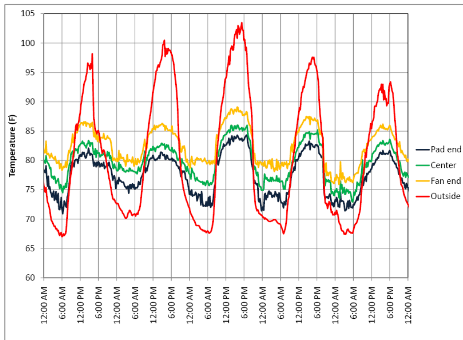
Figure 7. House temperatures in a house with attic inlets left “unlatched” when tunnel ventilating.
